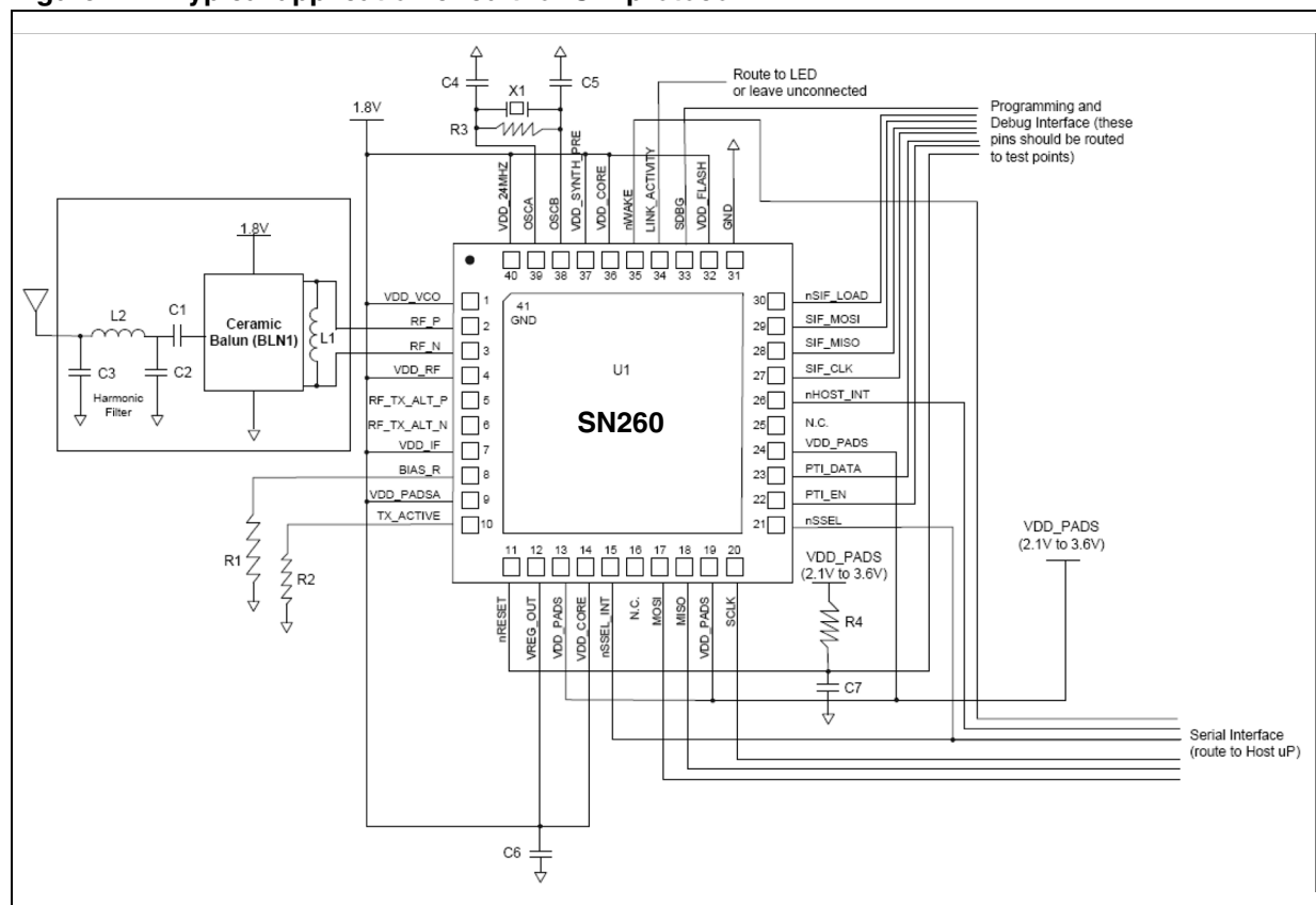
Figure 14. Typical application circuit for SPI protocol
