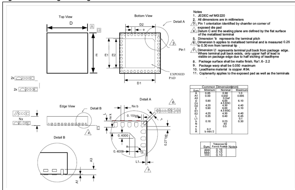
Figure 15. Package drawing
