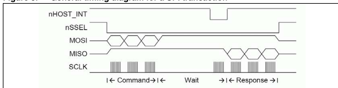
Figure 5. General timing diagram for a SPI transaction
